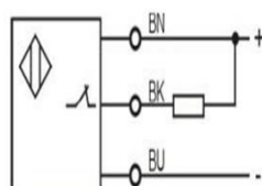
NPN NC
