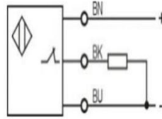
PNP NC
