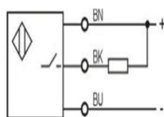
NPN NO
